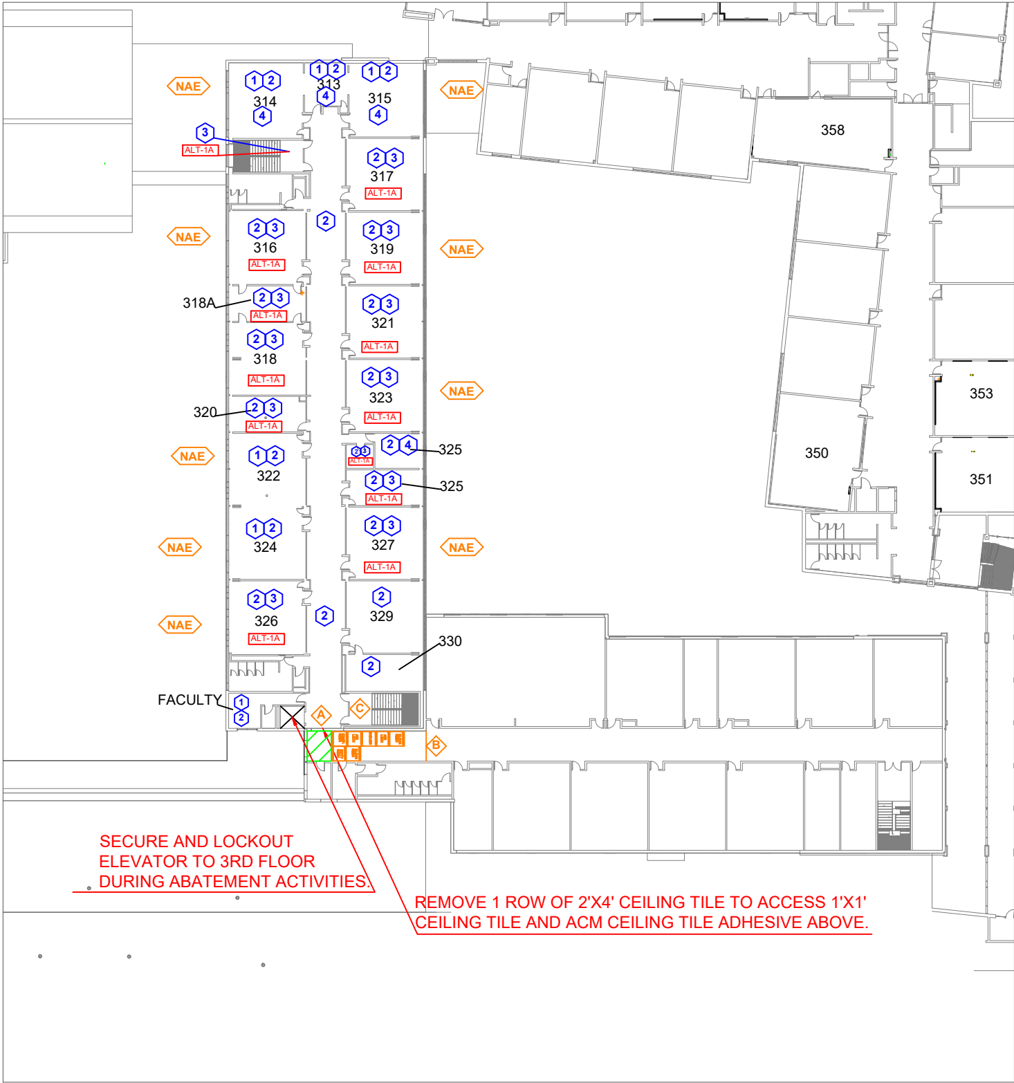
1 THIRD FLOOR CLASSROOMS, CORRIDOR, AND STAIRS ASB01 ASBESTOS ABATEMENT - 2021
