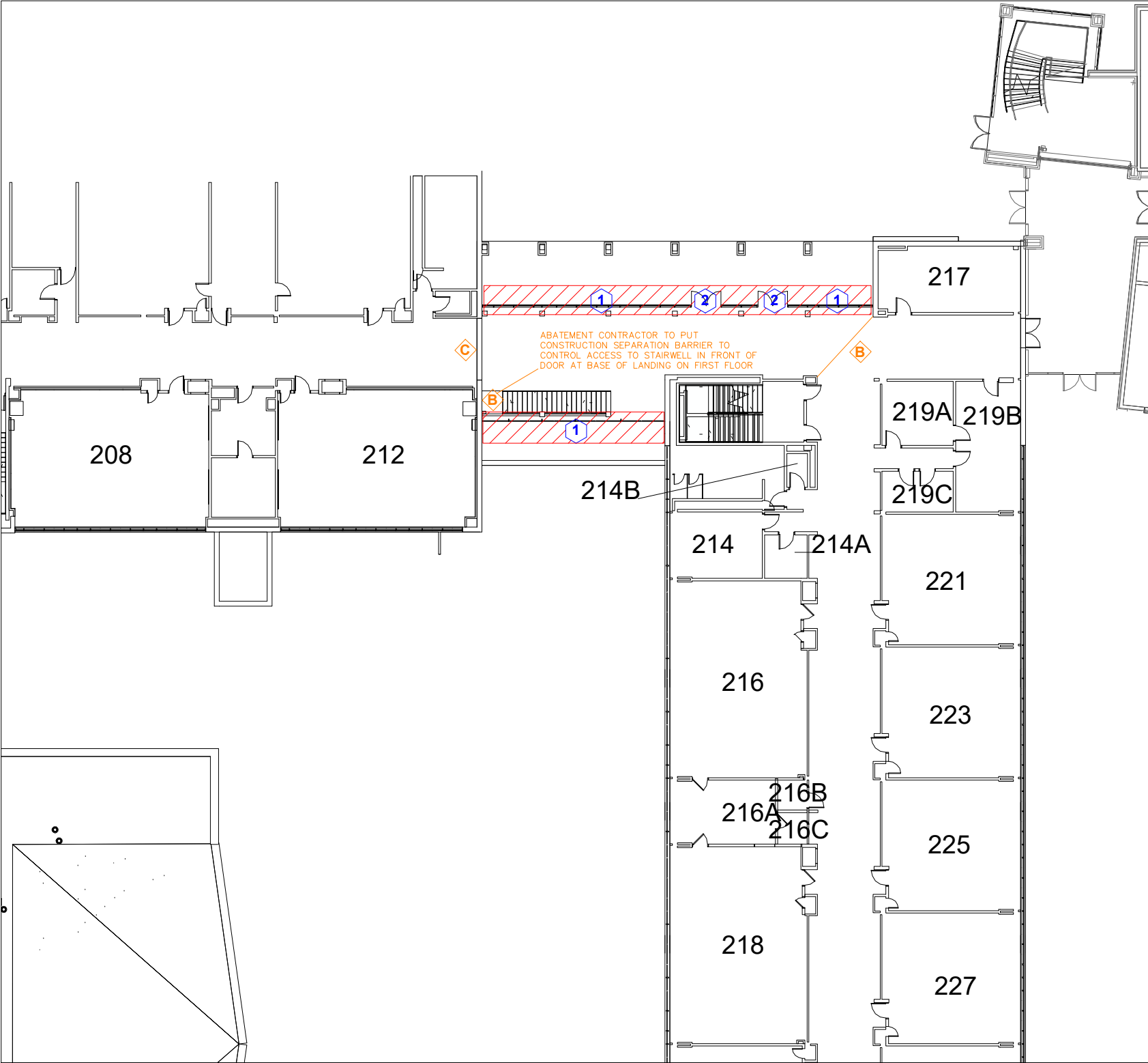
1 SECOND FLOOR EAHS02 ABATEMENT PLAN
